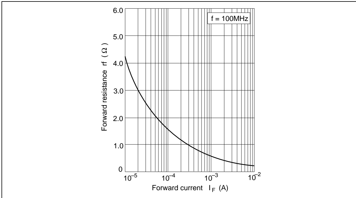
Fig.3 Forward resistance Vs. Forward current
